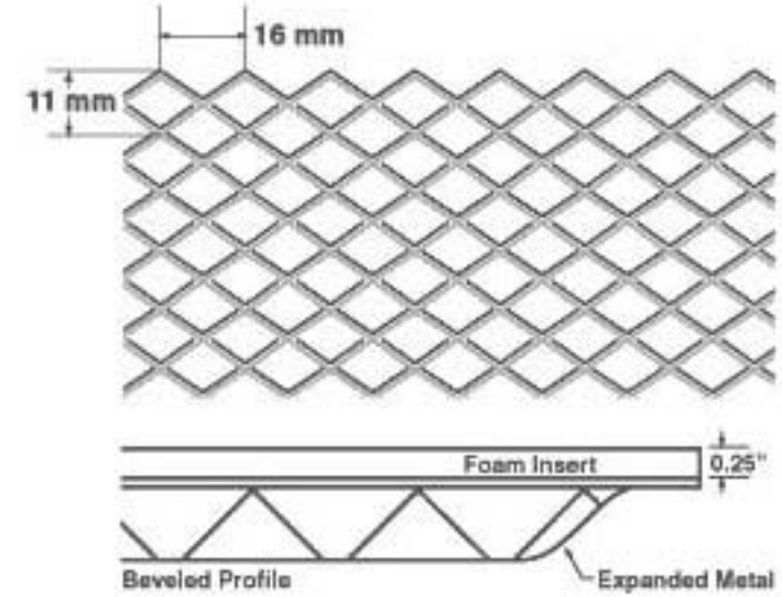
SQUARELINEstandard Dimension
