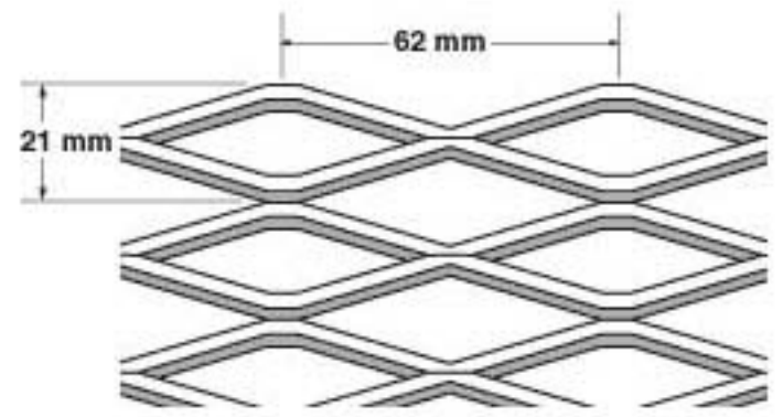
SQUARELINEUltra Dimension
