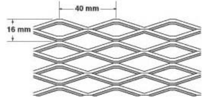
SQUARELINEmedium Dimension
